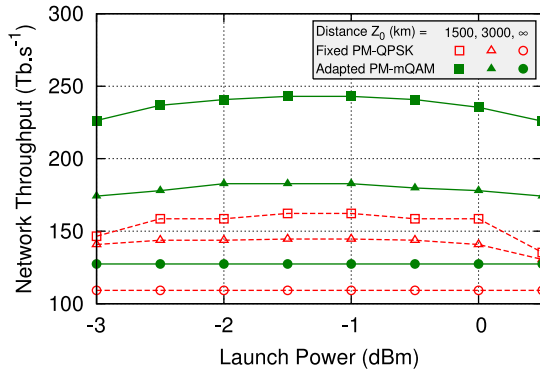
Fig. 8. The maximum network throughput for three characteristic traffic distances and for fixed PM-QPSK or route optimized PM-mQAM as a function of launch power, with the wavelength continuity constraint relaxed.
