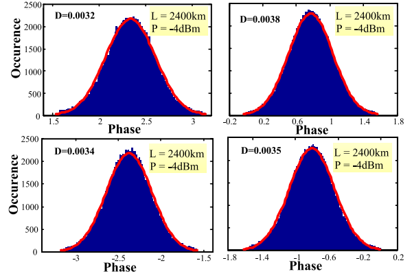
Fig. 3. Histogram of the received QPSK symbols' phase of the center channel in four quadrants of the constellation diagram.
