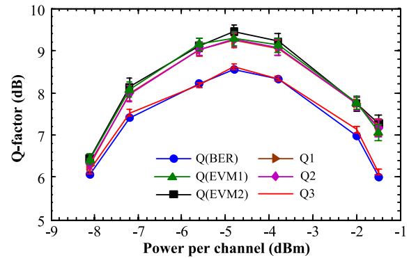
Fig. 5. Q-factor values for the #2 channel as a function of the launch power at 2400km.
